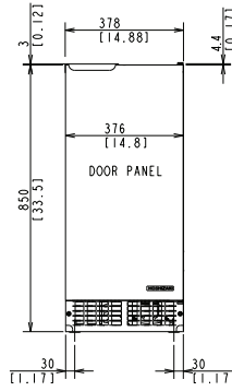
FRONT DIMENSIONS
