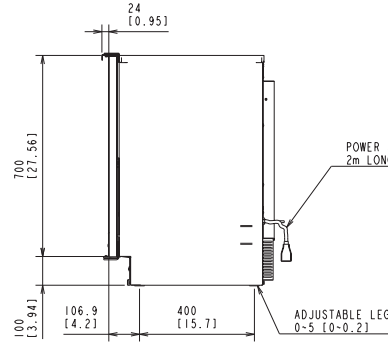
SIDE DIMENSIONS (ADA compliant unit)
